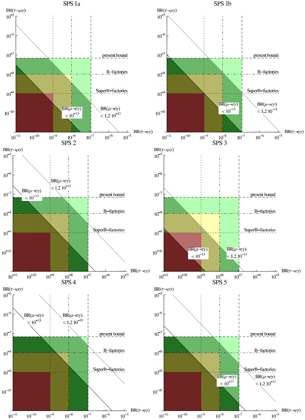
Figure 1: Allowed values for the branching ratios of the rare tau decays \tau \rightarrow e\gamma and \tau \rightarrow \mu\gamma from present experiments and from the bound BR(\mu \rightarrow e\gamma) \gtrsim C \times BR(\tau \rightarrow \mu\gamma)BR(\tau \rightarrow e\gamma) for the mSUGRA scenarios SPS1-5. The area in green indicates the observable window of present B -factories, and in yellow the observable window of future super B -factories. Excluded regions are shown with light shading, whereas allowed regions are shown with dark shading. In the plots it is assumed M_{\text{maj}} = 5 \times 10^{13} GeV.
