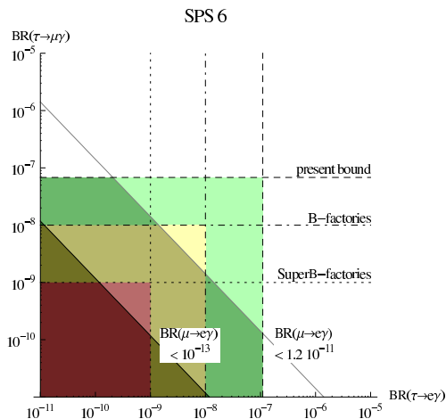
Figure 2: As in figure 1, but for the mSUGRA-like scenario SPS6.
